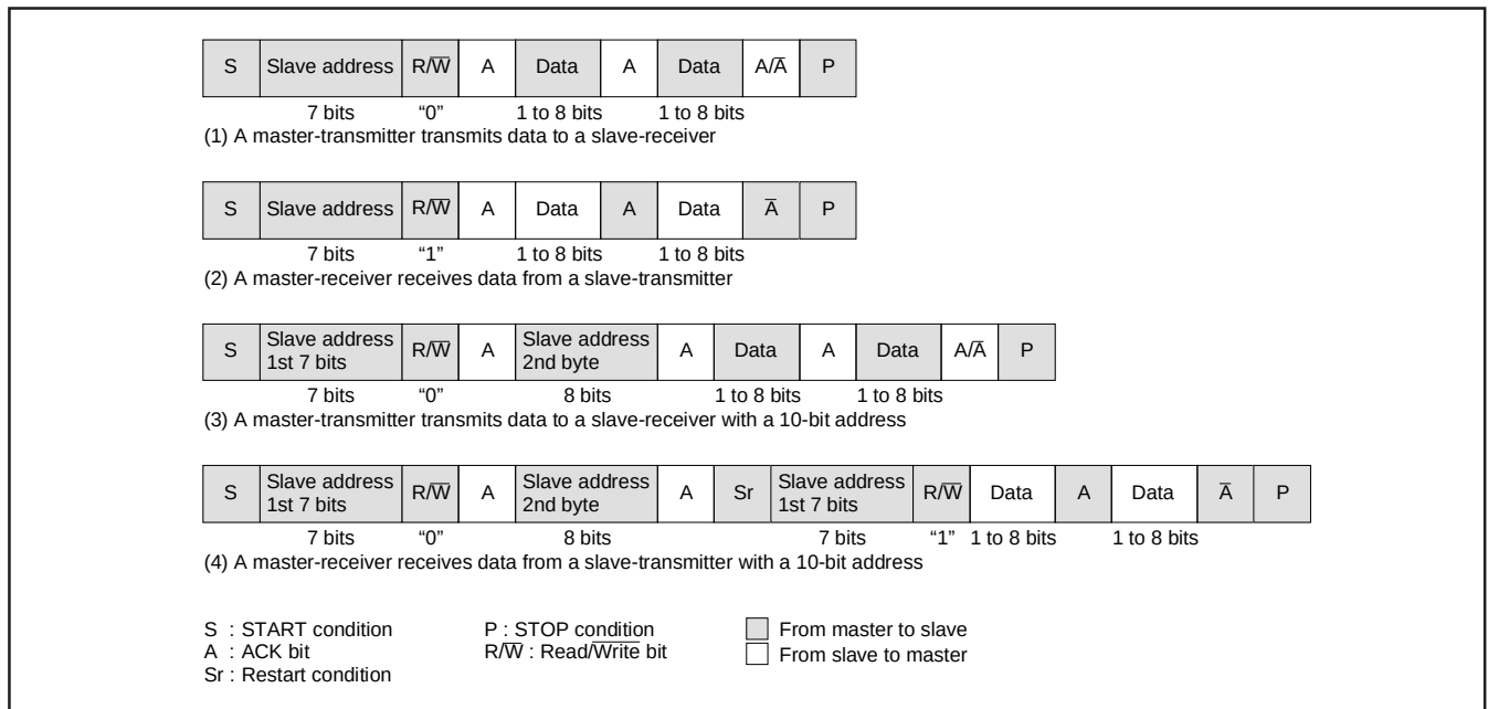
Fig. 8.6.12 Address Data Communication Format
