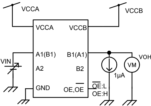
Figure 9 Test Circuit
