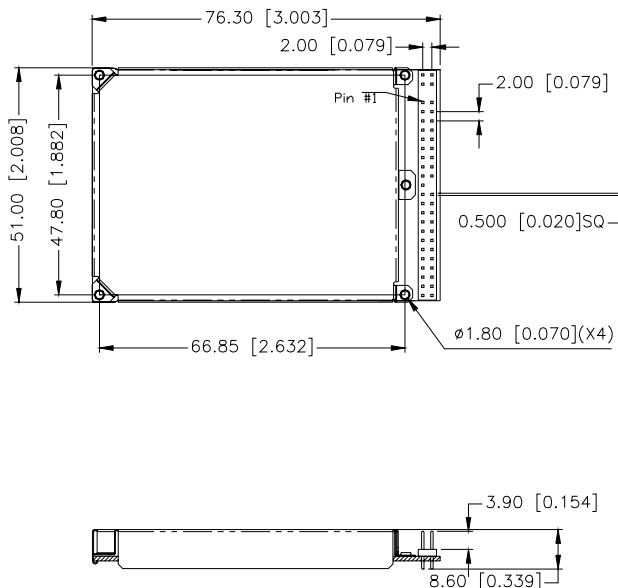
Figure 3: IDE 4000 1.8" Assembly
