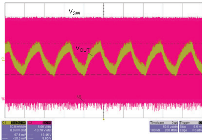
Figure 34: Output Voltage Ripple Amplitude Due to Dithering = 100 mV at V_{IN} = 12 V, and PWM Ratio = 100%
