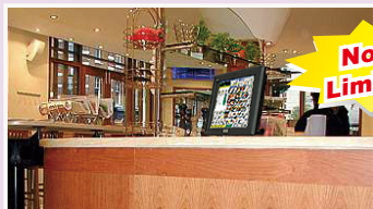
POS system
