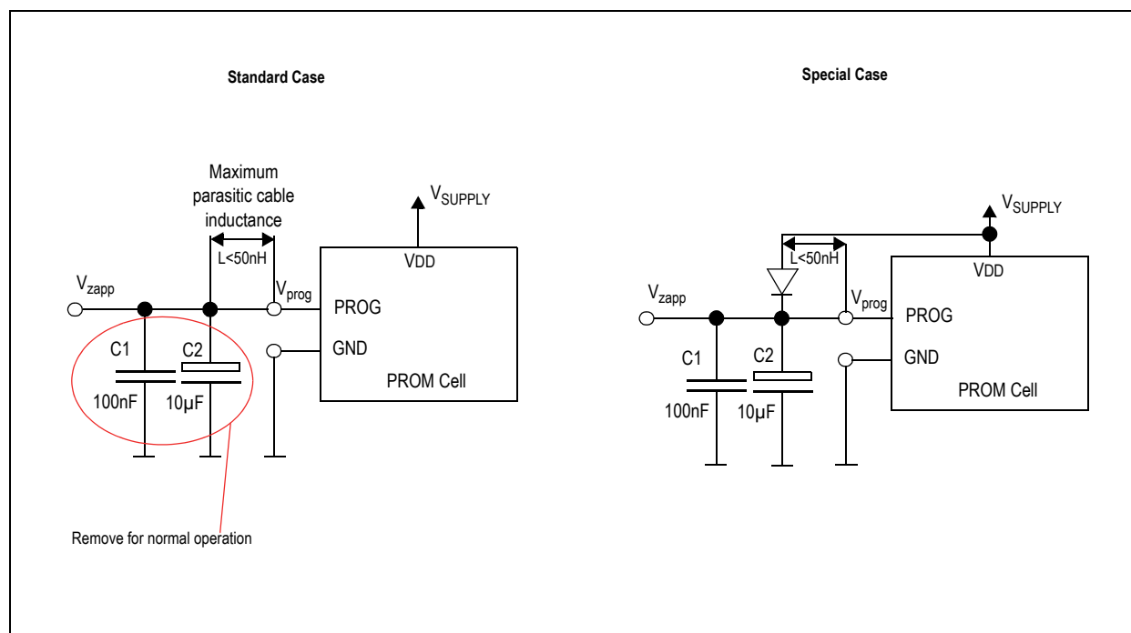
Figure 24: OTP Programming Connection
