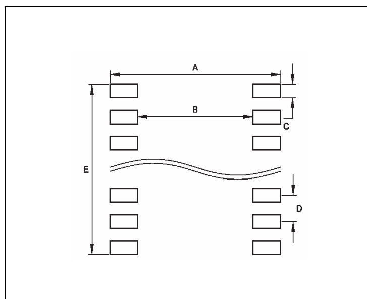
Figure 43: PCB Footprint
