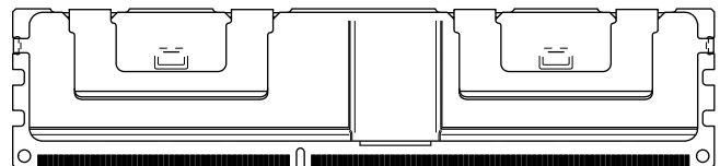
Figure 1: 240-Pin LRDIMM (MO-269 R/C A)
