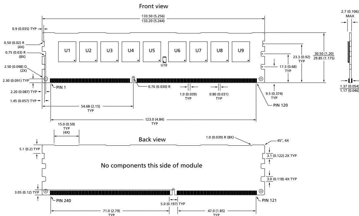
Figure 3: 240-Pin DDR3 UDIMM
