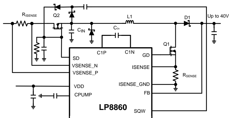
Figure 24. V_{\text{RAIL}} Multiplied by 4
