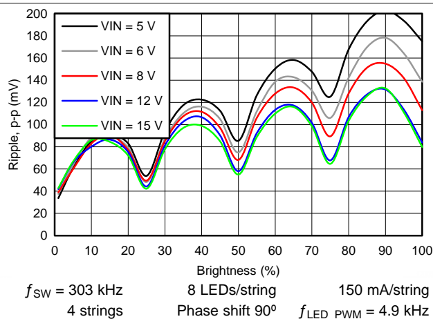
Figure 7. Boost Ripple
