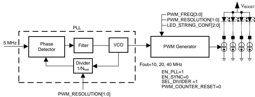
Figure 10. PWM Clocking With Internal Oscillator
