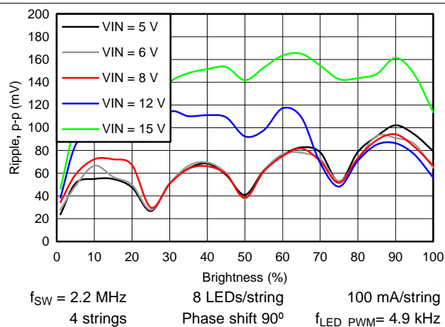
Figure 8. Boost Ripple
