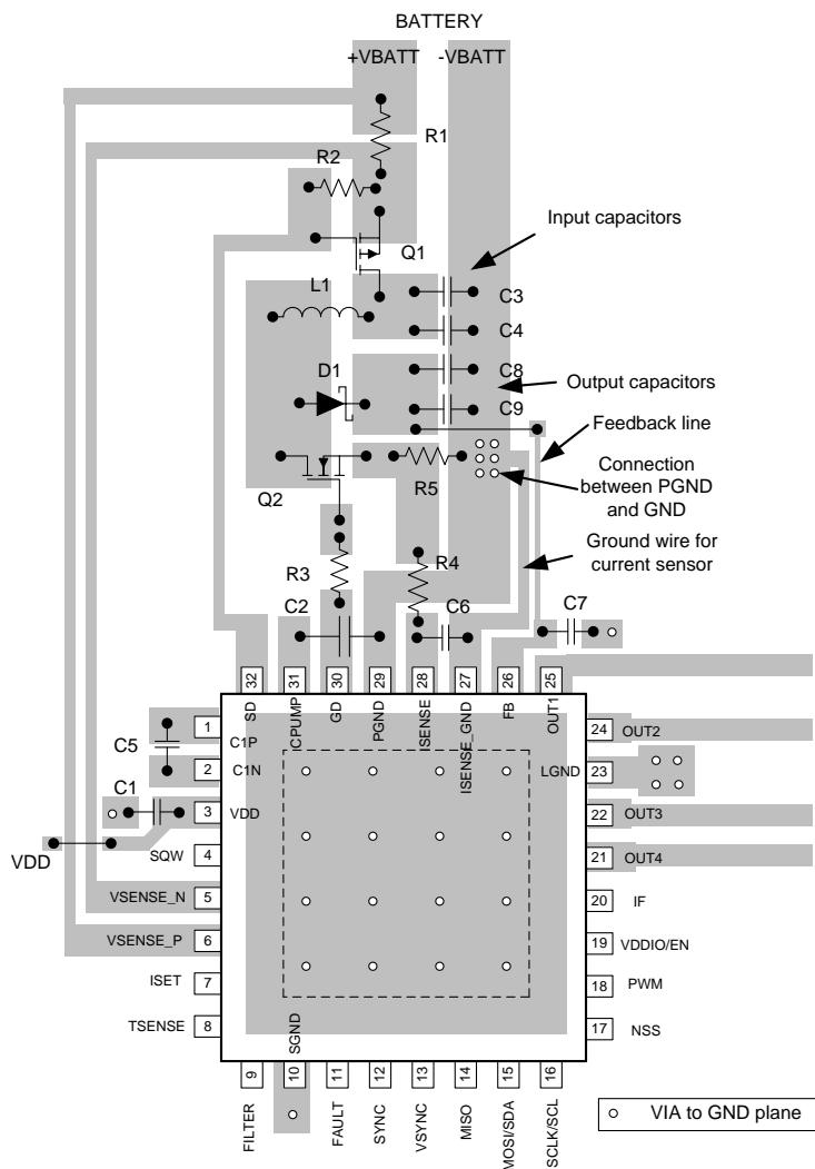
Figure 67. LP8860-Q1 Layout
