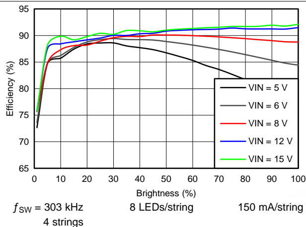
Figure 3. System Efficiency
