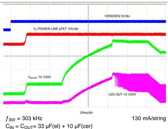
Figure 57. Typical Start-up
