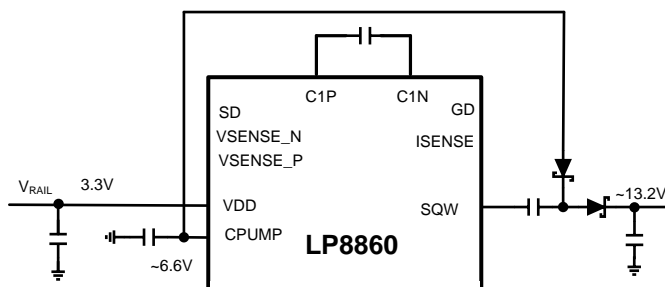
Figure 23. V_{\text{RAIL}} Multiplied by 2
