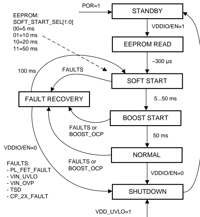
Figure 42. State Diagram
