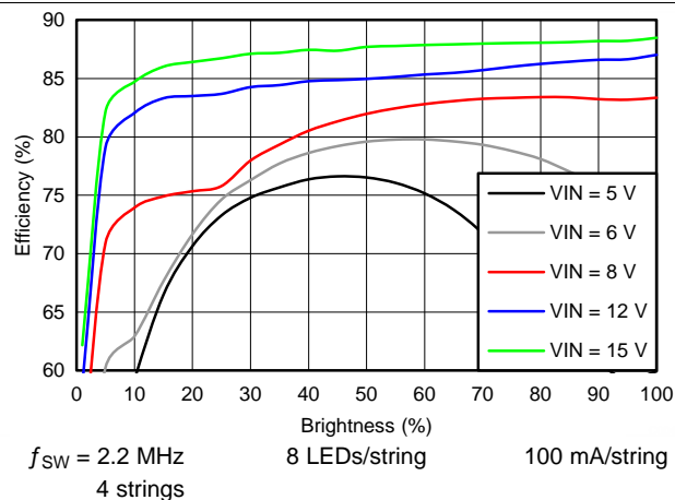
Figure 4. System Efficiency
