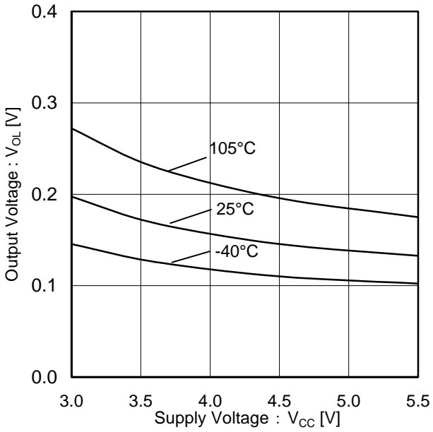
Figure 11. SEROUT Low Side Voltage ( V_{CC} characteristic @ I_O=4mA )
