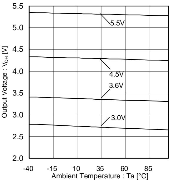
Figure 10. SEROUT High Side Voltage (Temperature characteristic @ I_O=-4mA )
