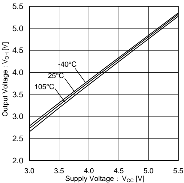
Figure 9. SEROUT High Side Voltage ( V_{CC} characteristic @ I_O=-4mA )
