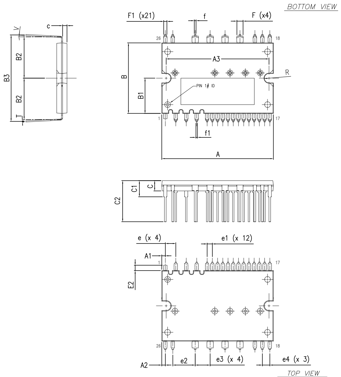
Figure 18. SDIP2F-26L type L package outline
