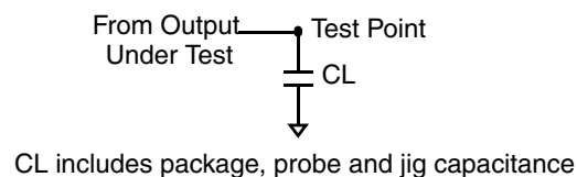
Figure 5. Load Circuit for Output Pin
