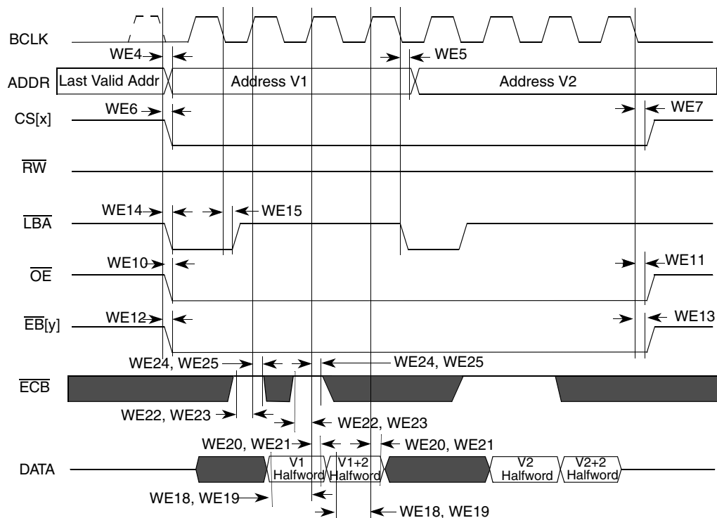
Figure 18. Synchronous Memory Timing Diagram for Two Non-Sequential Read Accesses— WSC = 2, SYNC = 1, DOL = 0
