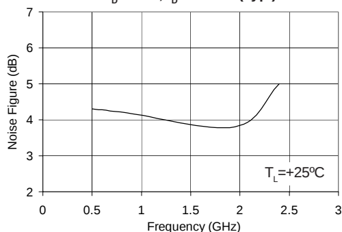
Noise Figure vs. Frequency V_D = 3.5\text{ V}, I_D = 60\text{ mA (Typ.)}
