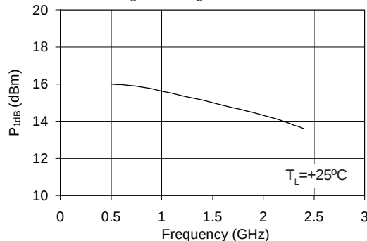
P 1dB vs. Frequency V_D = 3.5\text{ V}, I_D = 60\text{ mA (Typ.)}
