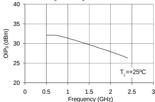
OIP 3 vs. Frequency V_D = 3.5\text{ V}, I_D = 60\text{ mA (Typ.)}
