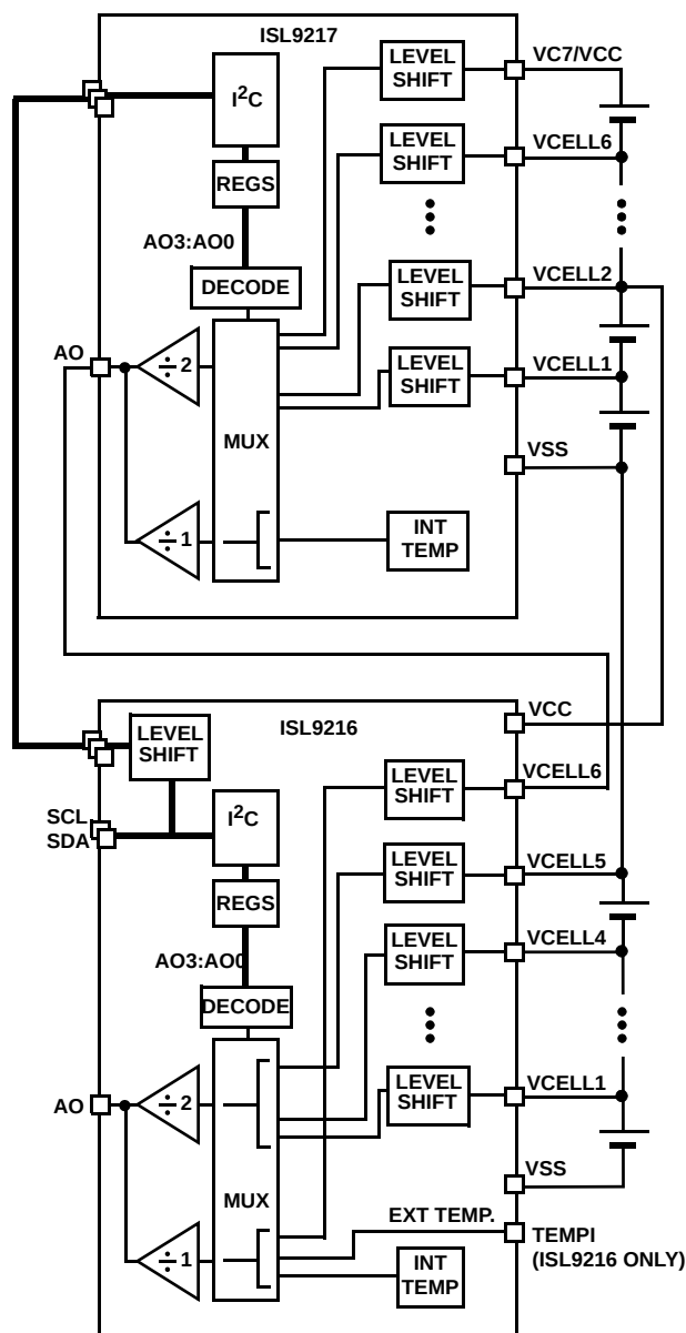
FIGURE 6. ANALOG OUTPUT MONITORING DIAGRAM
