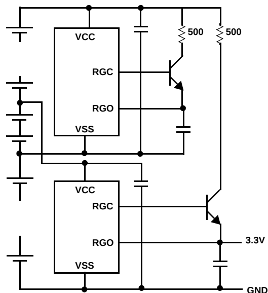
FIGURE 2. VOLTAGE REGULATOR CIRCUITS
