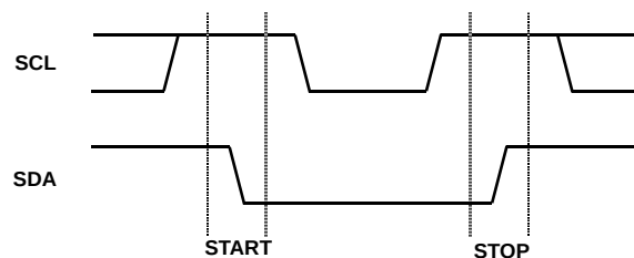
FIGURE 10. I 2 C START AND STOP BITS
