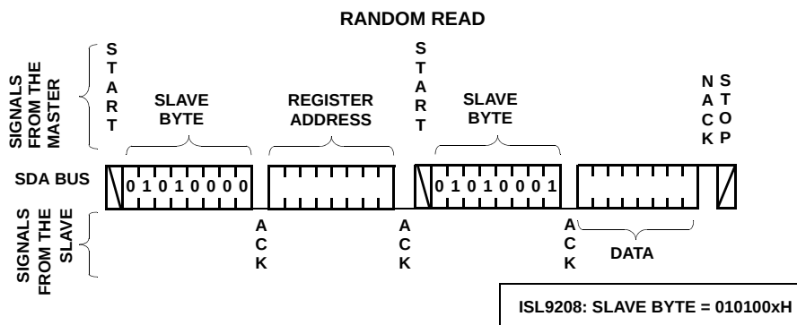
FIGURE 13. READ SEQUENCE
