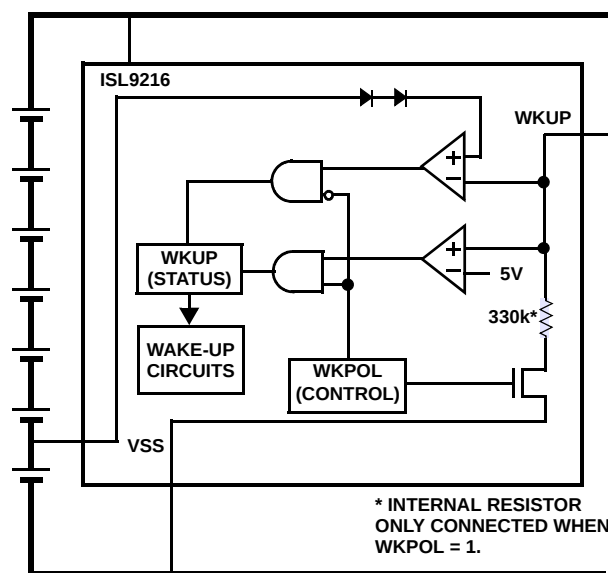
FIGURE 3. WAKE-UP CONTROL CIRCUITS
