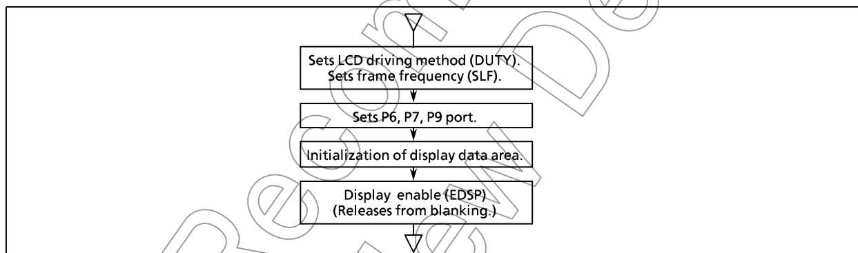
Figure 2-51. Initial Setting of LCD Driver
