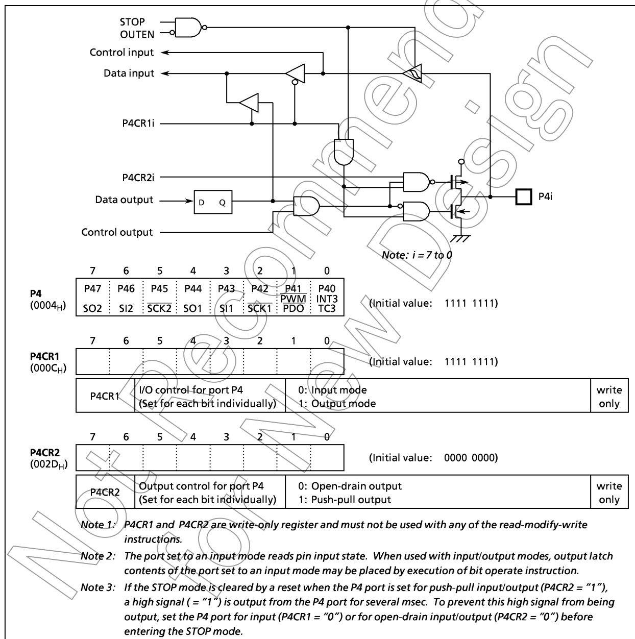
Figure 2-6. Port P4
