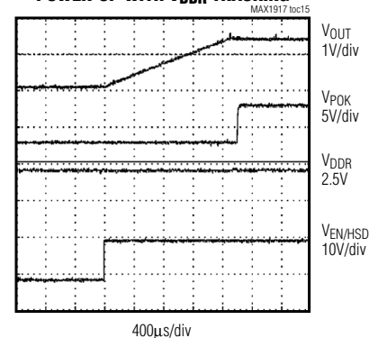
POWER-UP WITH VDD TRACKING
