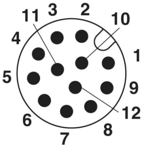
Schematic diagram
