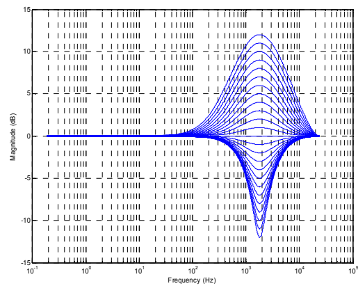
Figure 60 EQ Band 4 – Peak Filter Gains for Lowest Cut-off Frequency, EQ4BW=0
