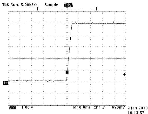
Figure 6. 5-Ω Load
