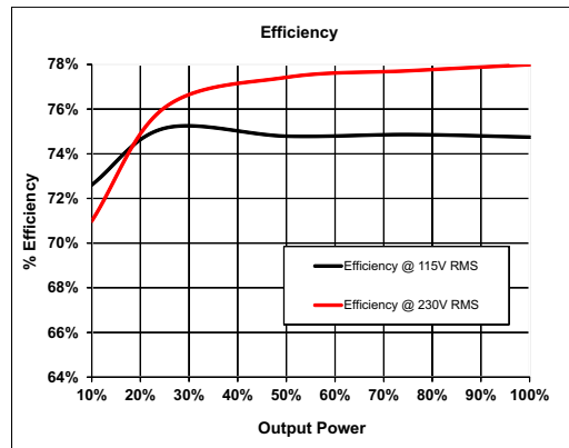
Figure 3. UCC28720EVM-212 Efficiency
