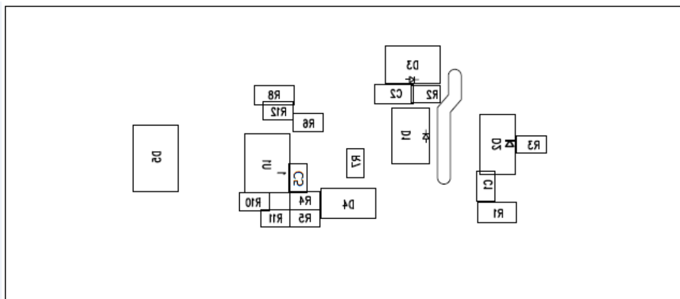
Figure 15. Bottom Assembly Drawing
