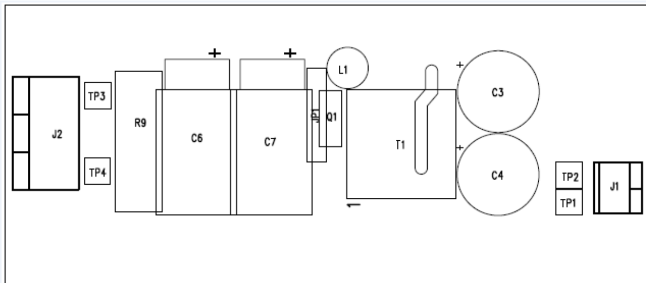
Figure 13. Top Assembly Drawing
