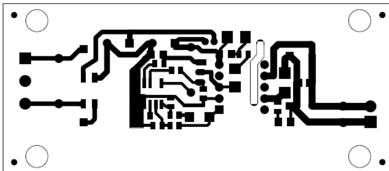
Figure 16. PCB Assembly Drawing
