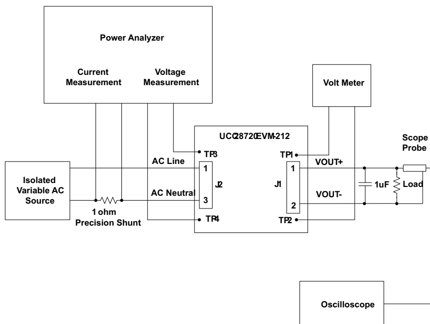
Figure 2. UCC28720EVM-212 Test Setup
