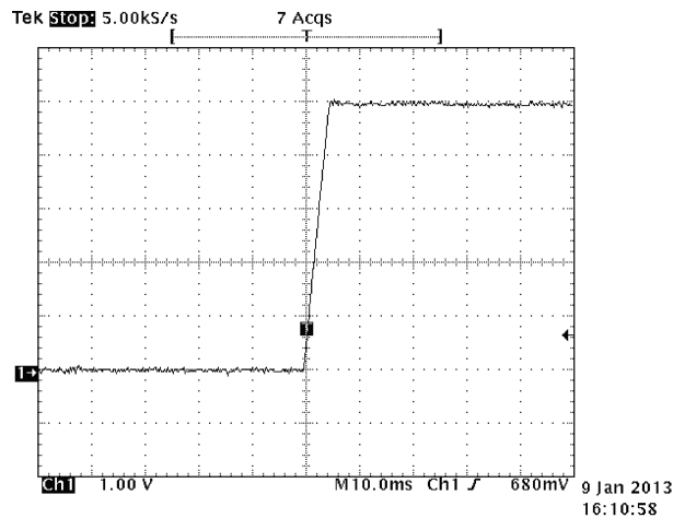
Figure 4. Output Ripple Voltage at Full Load
