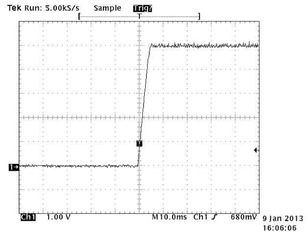
Figure 5. No Load
