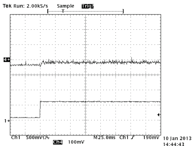
Figure 8. 5-Ω Load
