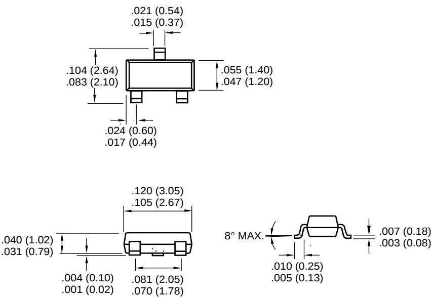
3-Pin SOT-23B (JEDEC TO-236)
