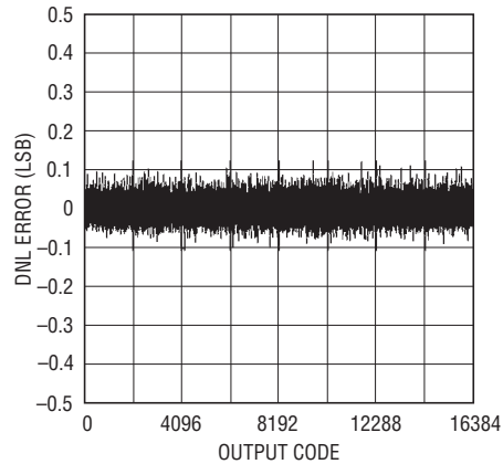
LTM9008-14: Differential Nonlinearity (DNL) vs Output Code
