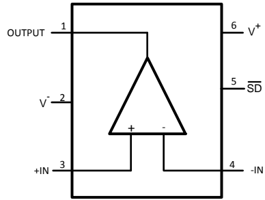
Figure 2. SOT-23-6 Top View
