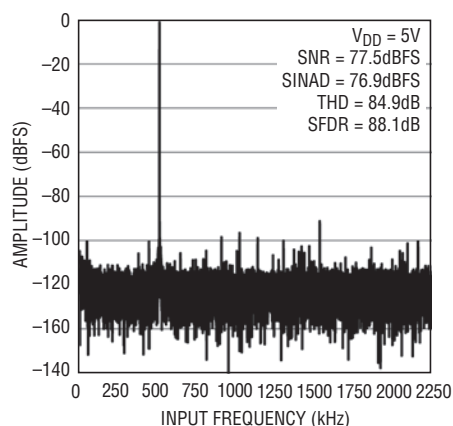
32k Point FFT, f_S = 4.5\text{Mps} f_{\text{IN}} = 500\text{kHz}
