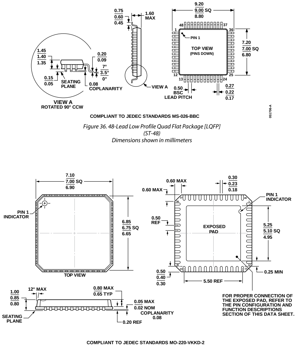
Figure 37. 48-Lead Lead Frame Chip Scale Package [LFCSP_VQ] 7 mm × 7 mm Body, Thin Quad (CP-48-1) Dimensions shown in millimeters
