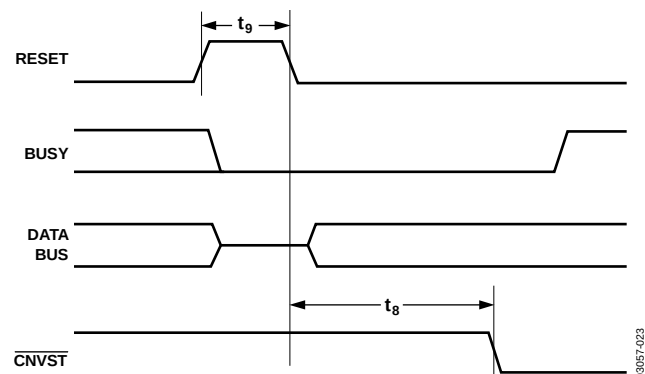
Figure 24. Reset Timing
