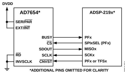
Figure 35. Interfacing the AD7654 to an SPI Interface
