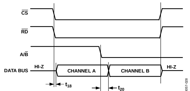
Figure 29. A/B Channel Reading
