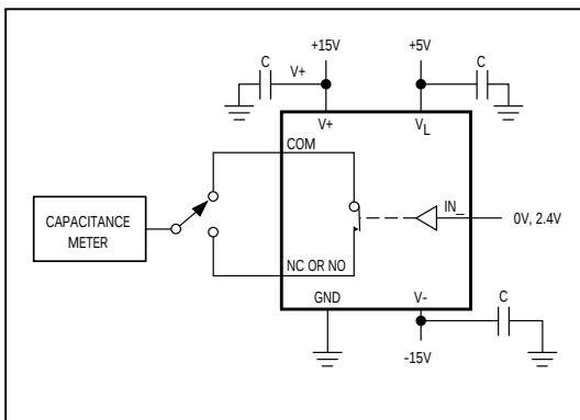
Figure 7. Channel-Off Capacitance
