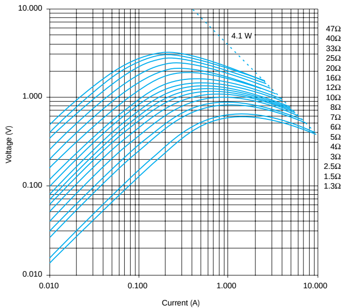
TYPICAL VOLTAGE/CURRENT CHARACTERISTICS FOR TYPE NF15
