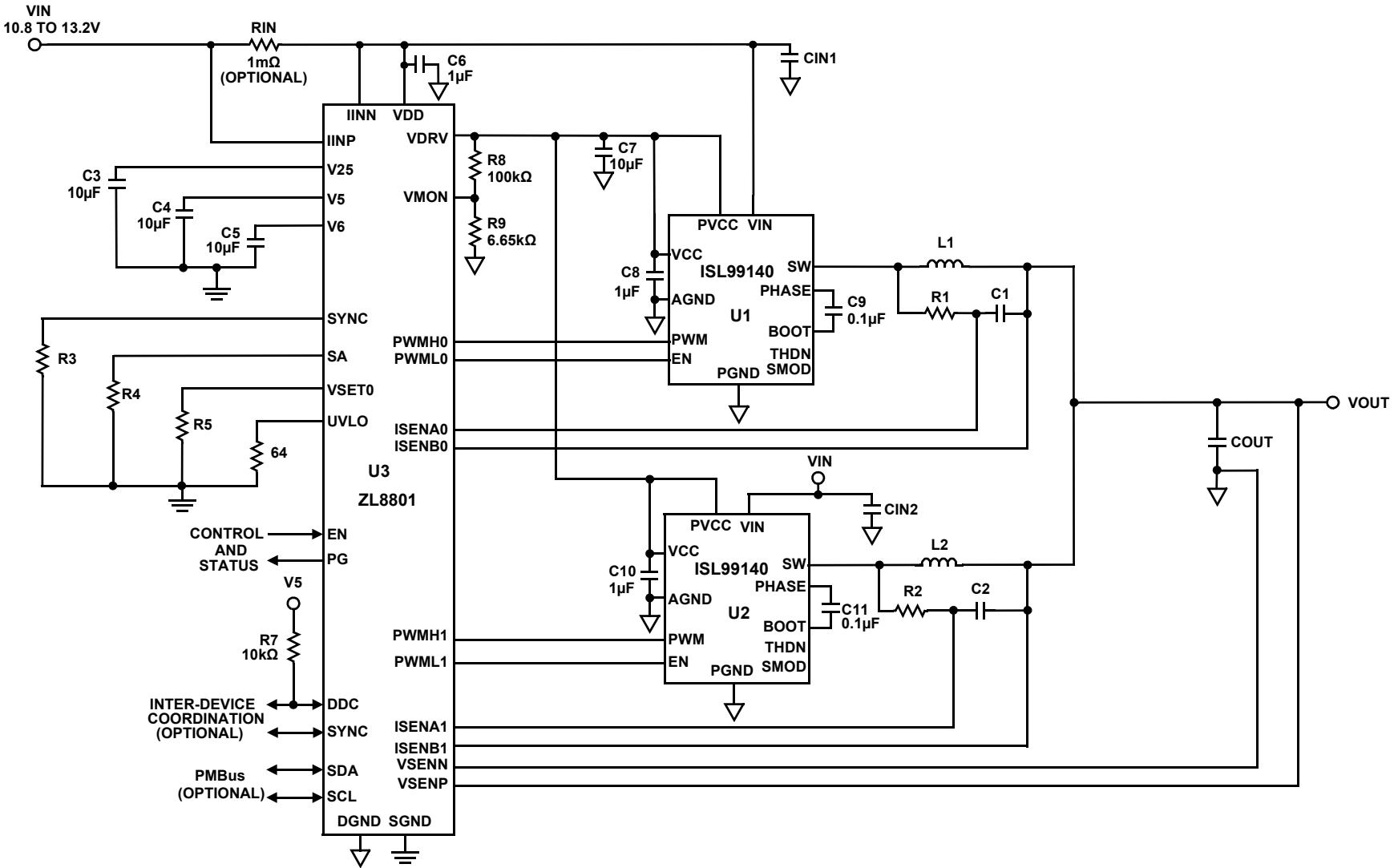
FIGURE 3. ZL8801 SCHEMATIC
