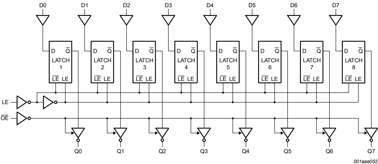
Fig. 5. Logic diagram
