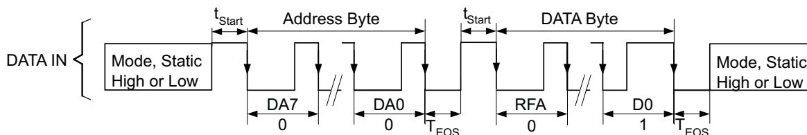
Figure 14. EasyScale Protocol Without Acknowledge (RFA=0)
