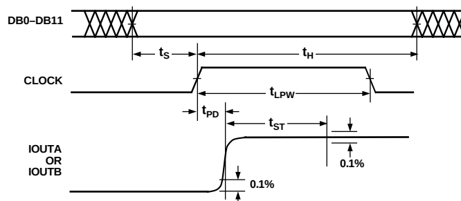
Figure 1. Timing Diagram
