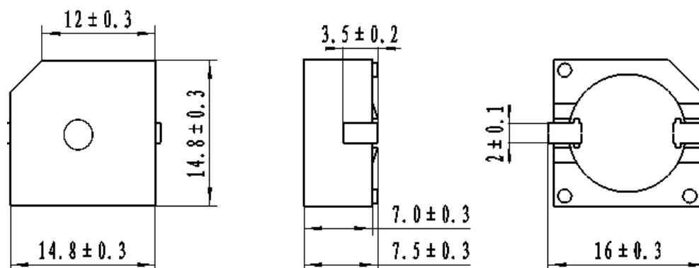
Suggested Pad PCB-Layout
