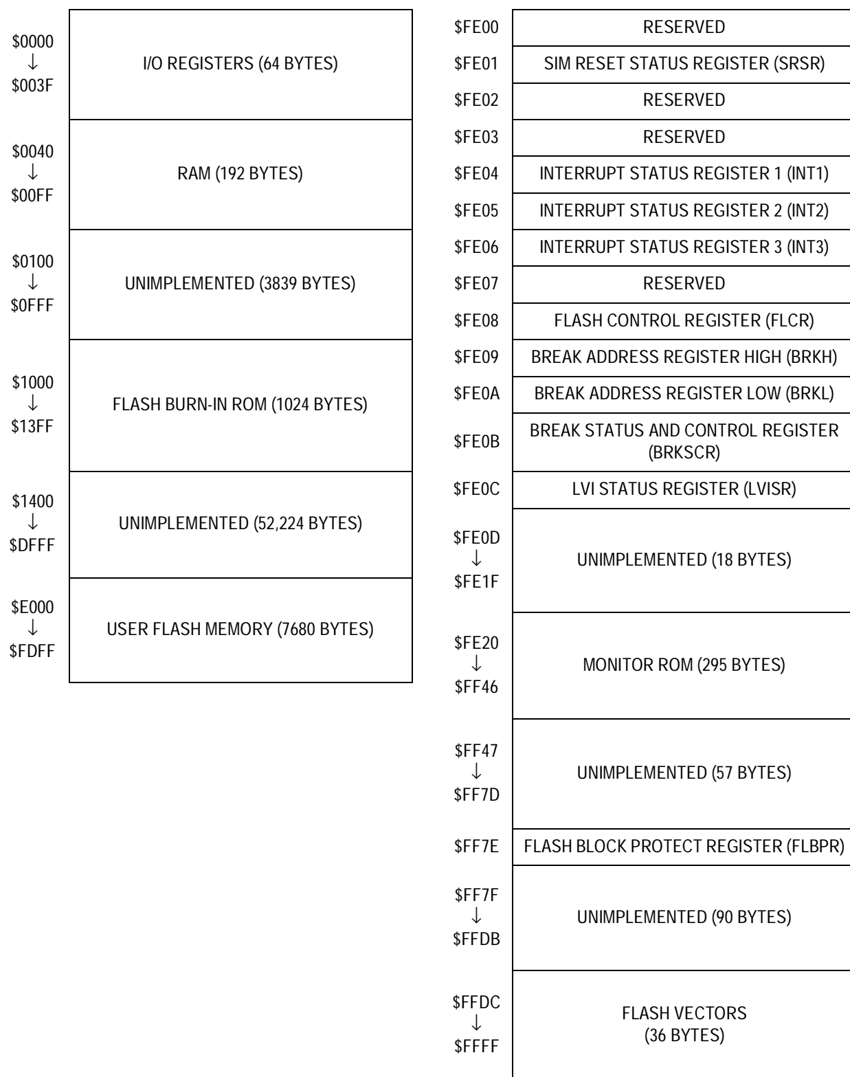
Figure 2-1. Memory Map
