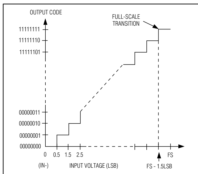
Figure 9. ADC Input/Output Transfer Function
