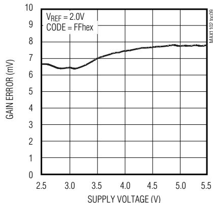
DAC GAIN ERROR vs. SUPPLY VOLTAGE
