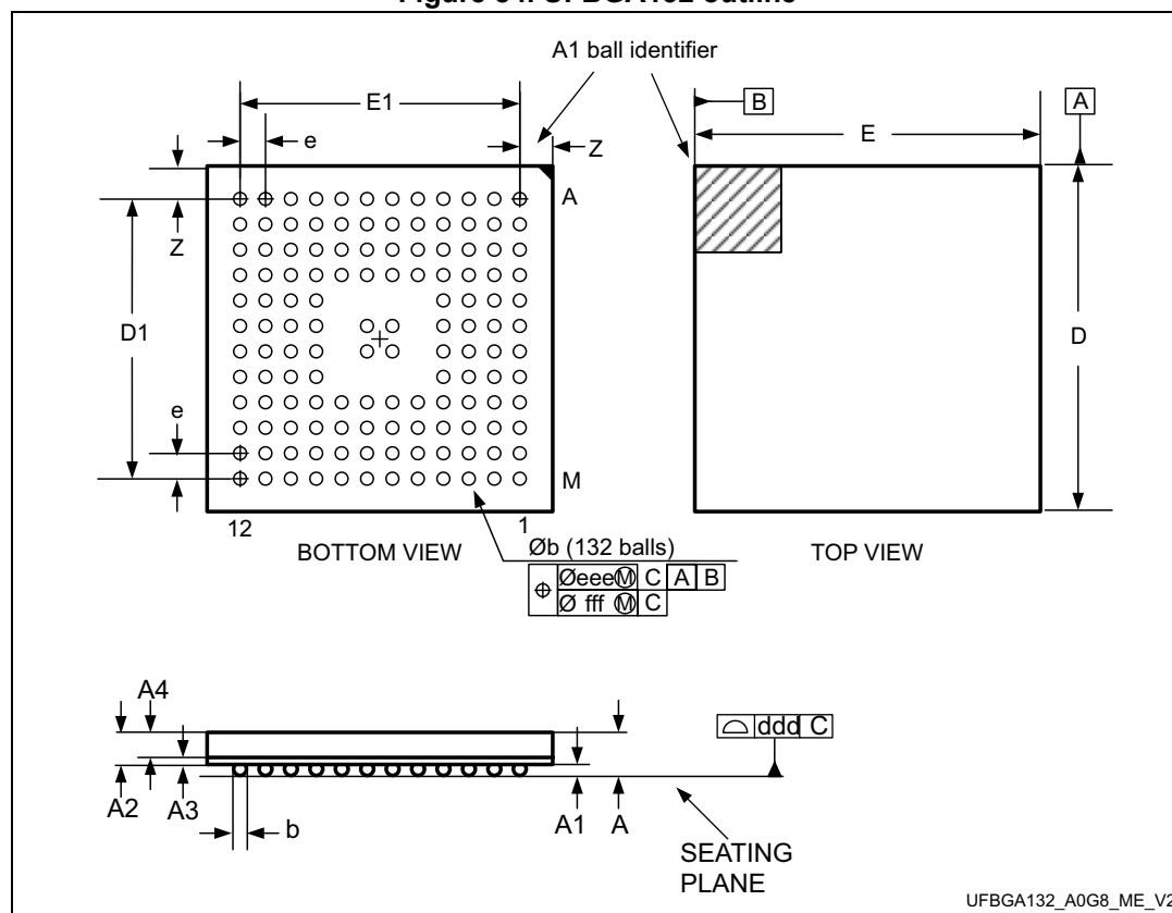
Figure 84. UFBGA132 outline
