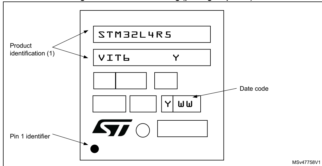
Figure 89. LQFP100 marking (package top view)
