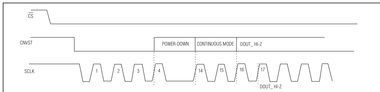
Figure 8. Dual-Output CNVST Transition Modes
