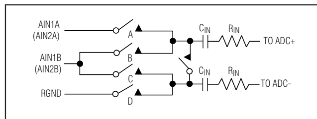
Figure 3. Equivalent Input Circuit
