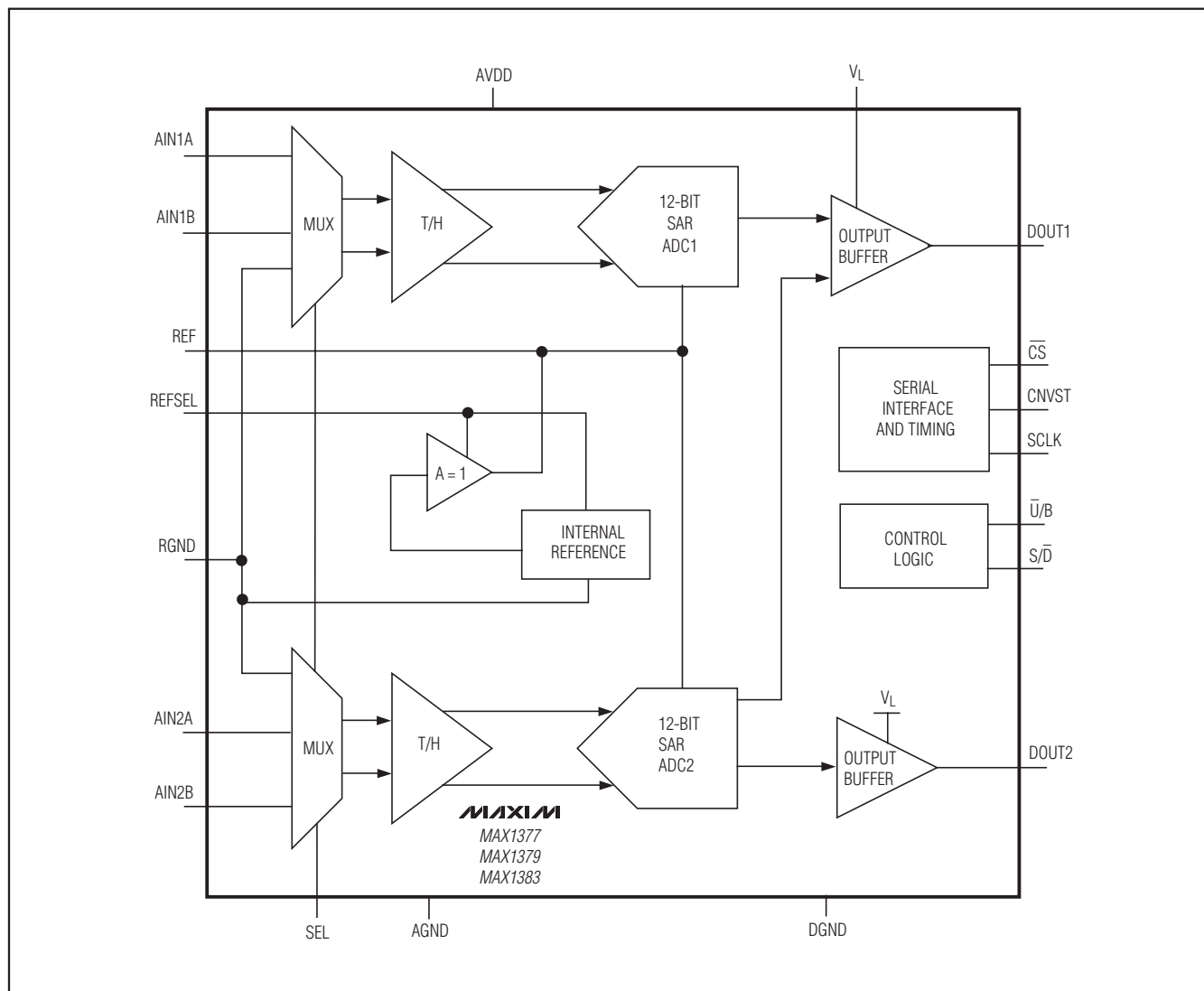
Functional Diagram
