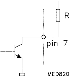
Fig.8 50/60 Hz output.
