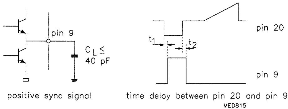
Fig.3 Sync output.
