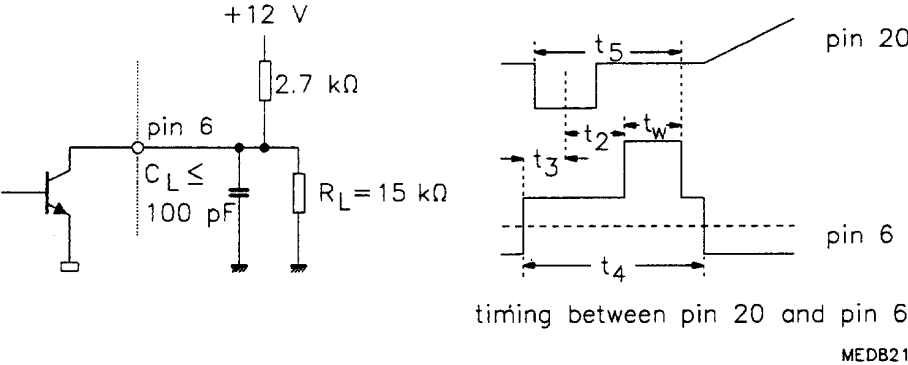
Fig.9 Sandcastle output.
