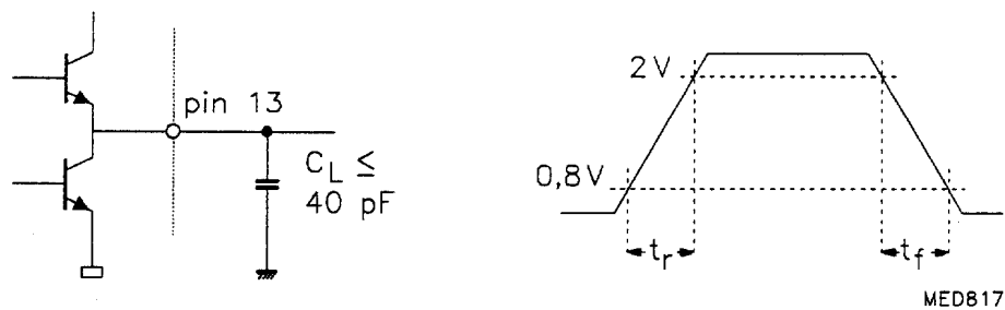
Fig.5 Clock output.
