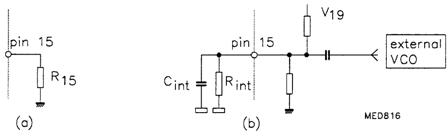
Fig.4 Pin 15 circuit for (a) internal VCO; (b) external VCO.
