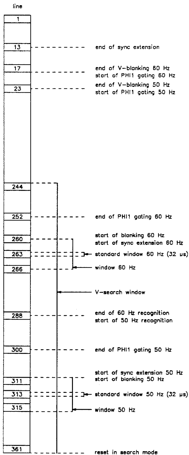
Fig.17 V-timing.
