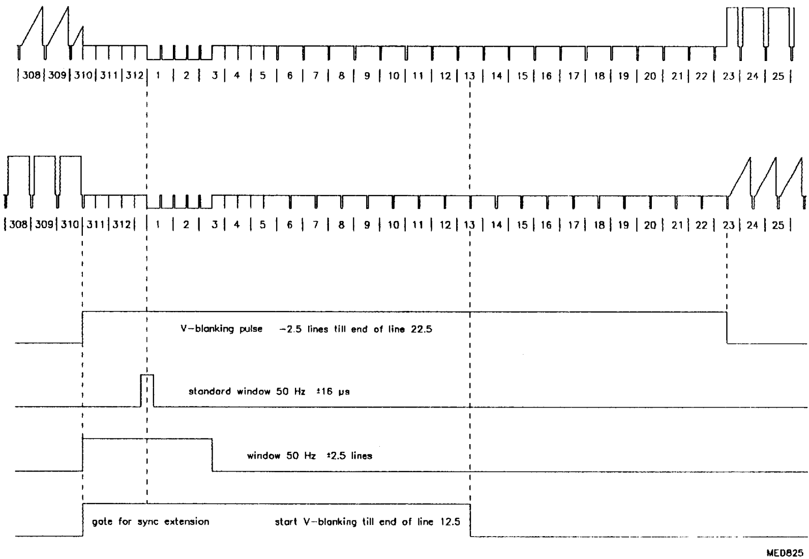
Fig.13 V-timing at 50 Hz operation.
