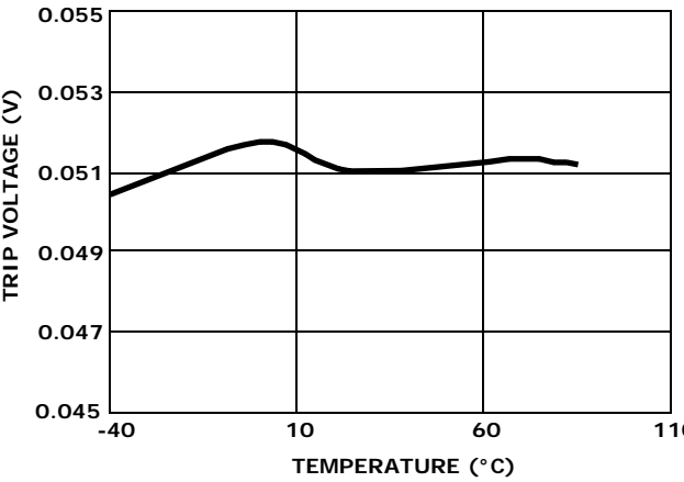
FIGURE 25. SENSE TRIP VOLTAGE
