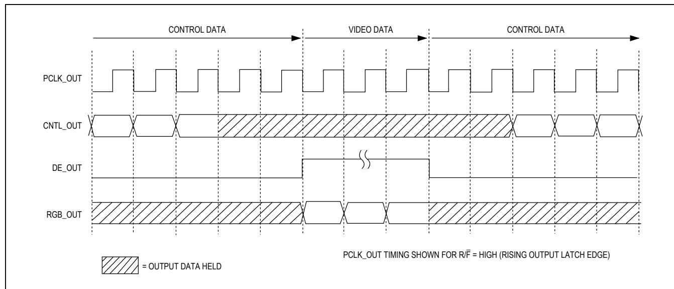
Figure 18. Output Timing
