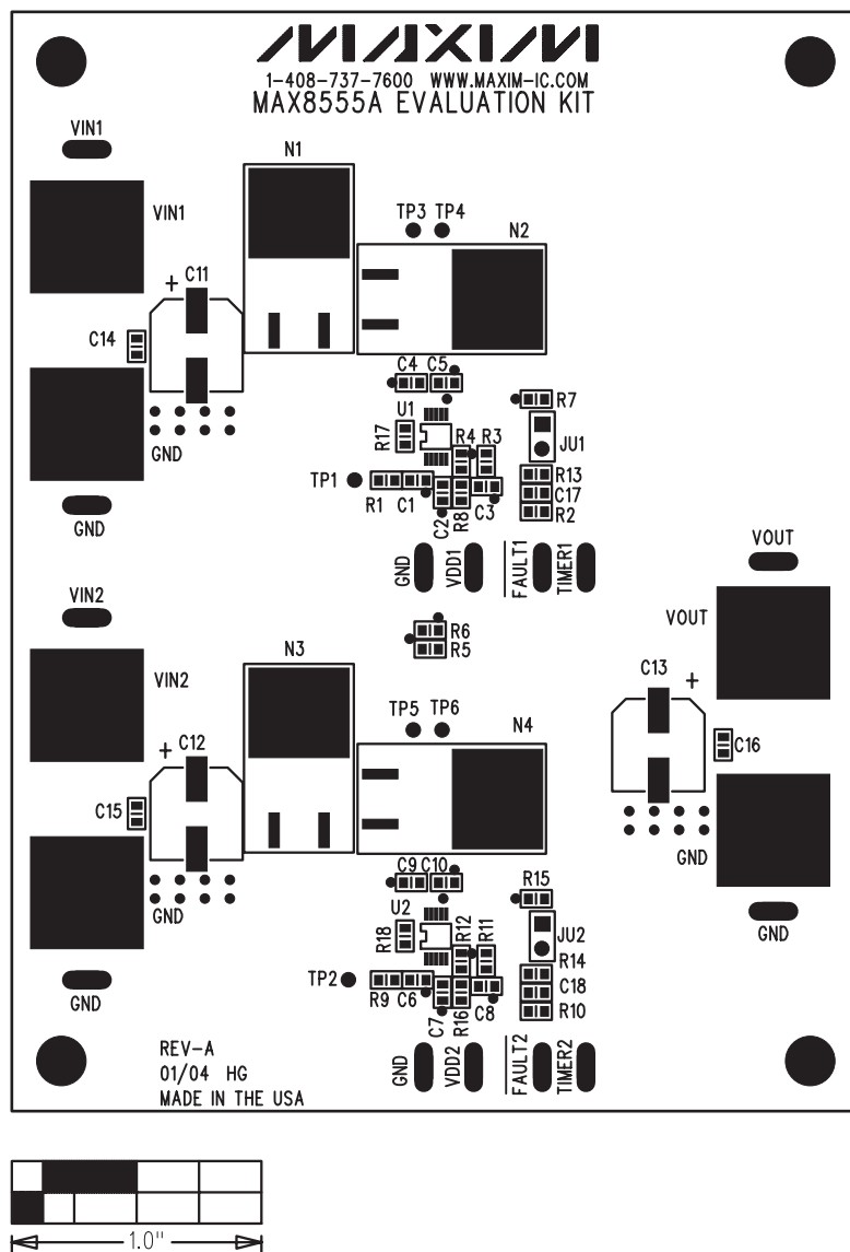
Figure 2. MAX8555A EV Kit Component Placement Guide—Component Side
