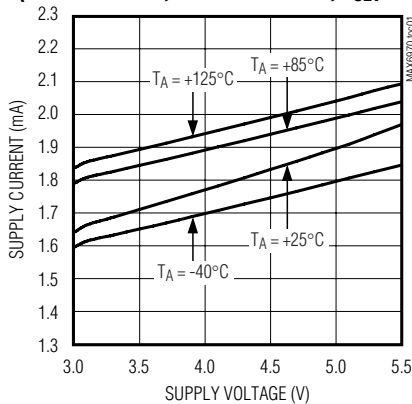
SUPPLY CURRENT vs. SUPPLY VOLTAGE (INTERFACE IDLE, ALL OUTPUTS OFF, R_{SET} = 720\Omega )
