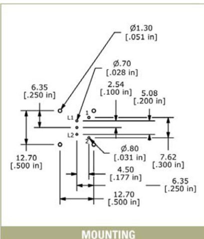
MOUNTING
