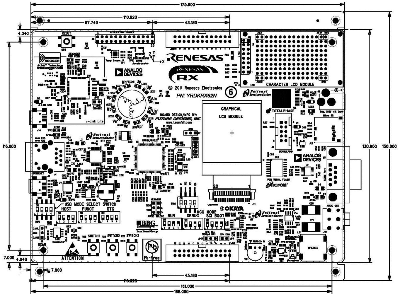
Figure 4-2: Board Dimensions
