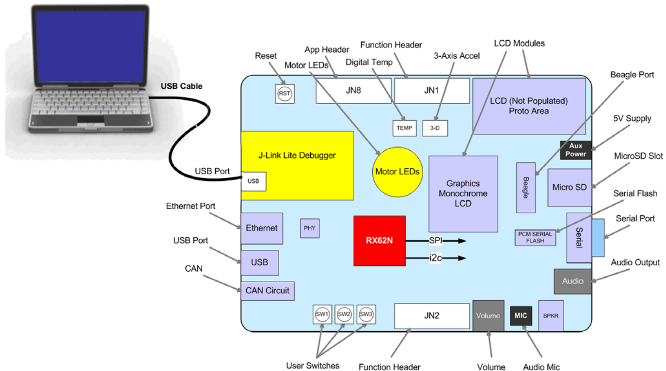
Figure 5-2: RDK Connections
