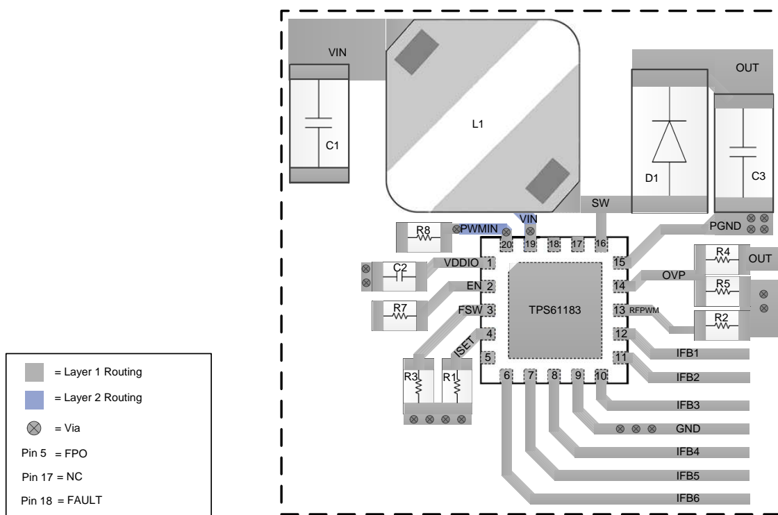
Figure 21. TPS61183 Layout
