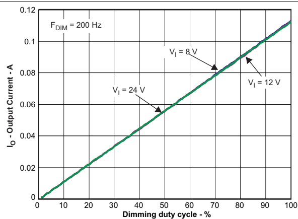
Figure 2. Dimming Linearity
