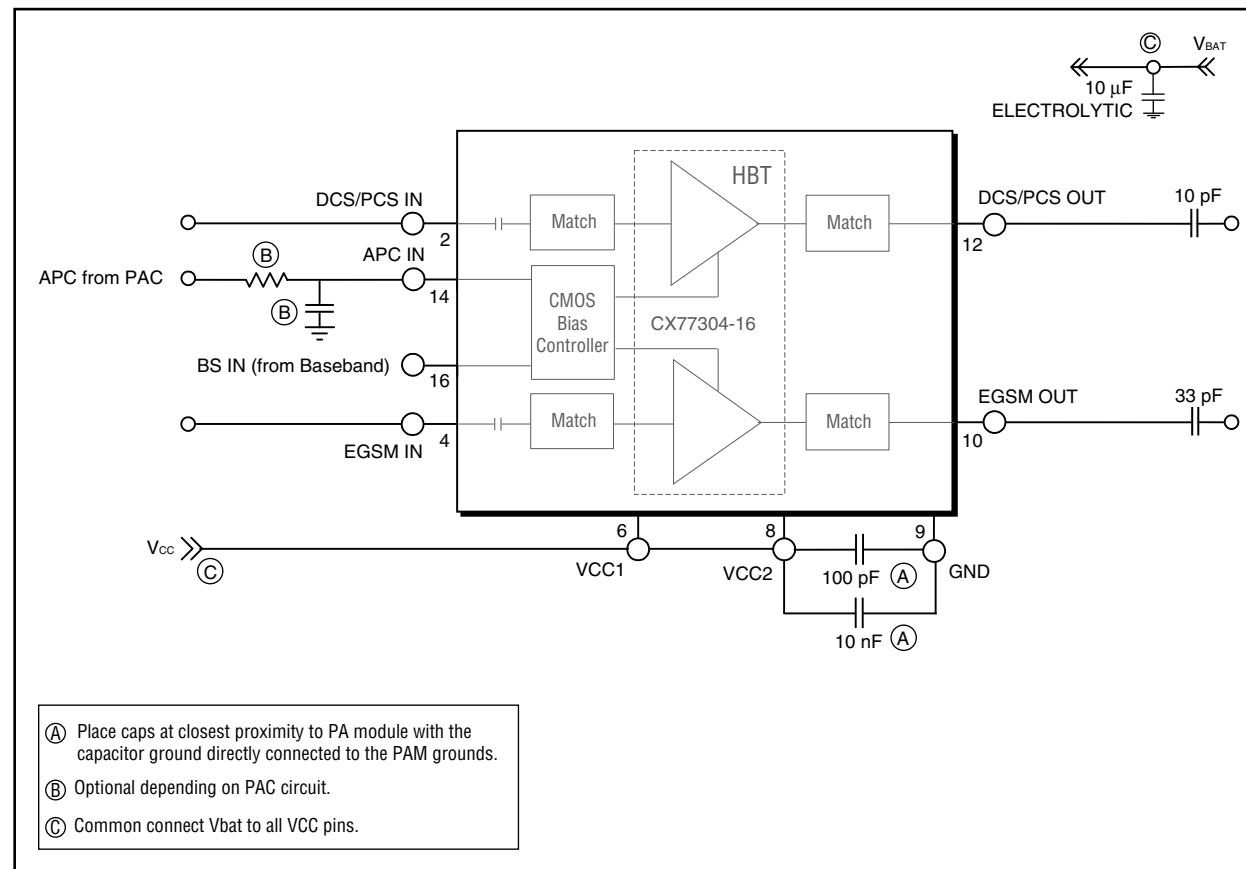
Figure 1. Typical CX77304-16 PAM Application
