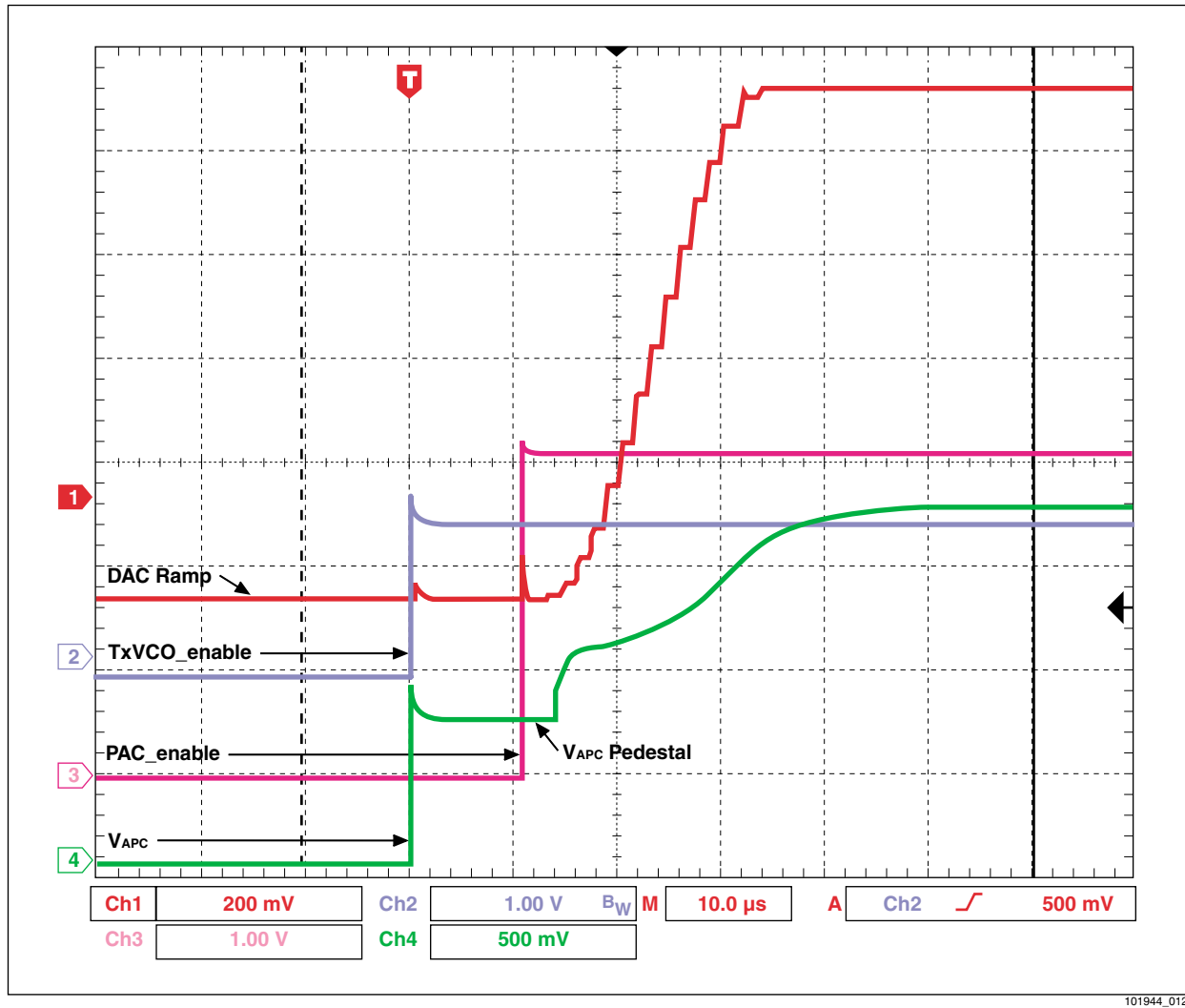
Figure 14. GSM Transmitter - Typical Ramp-up Signals
