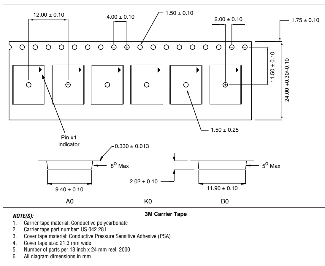
Figure 6. CX77304-16 Tape and Reel Dimensions
