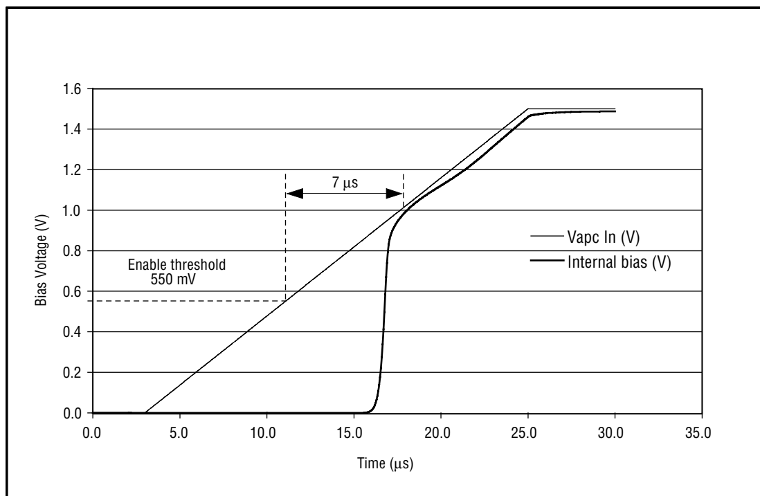
Figure 12. PAM Internal Bias Performance – No Pedestal Applied
