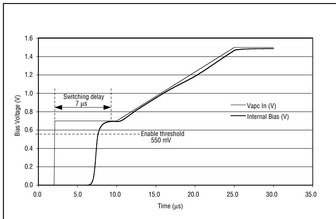
Figure 13. PAM Internal Bias Performance – Pedestal Applied
