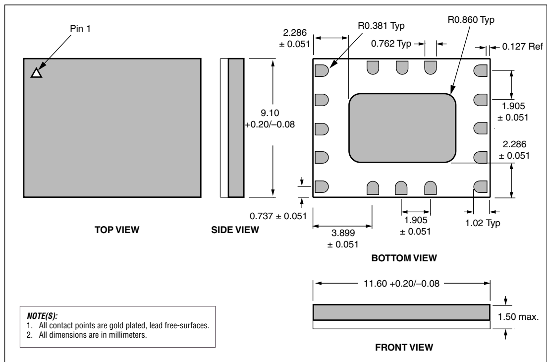
Figure 2. CX77304-16 PAM Package Dimensions–16-pin Module (All Views)
