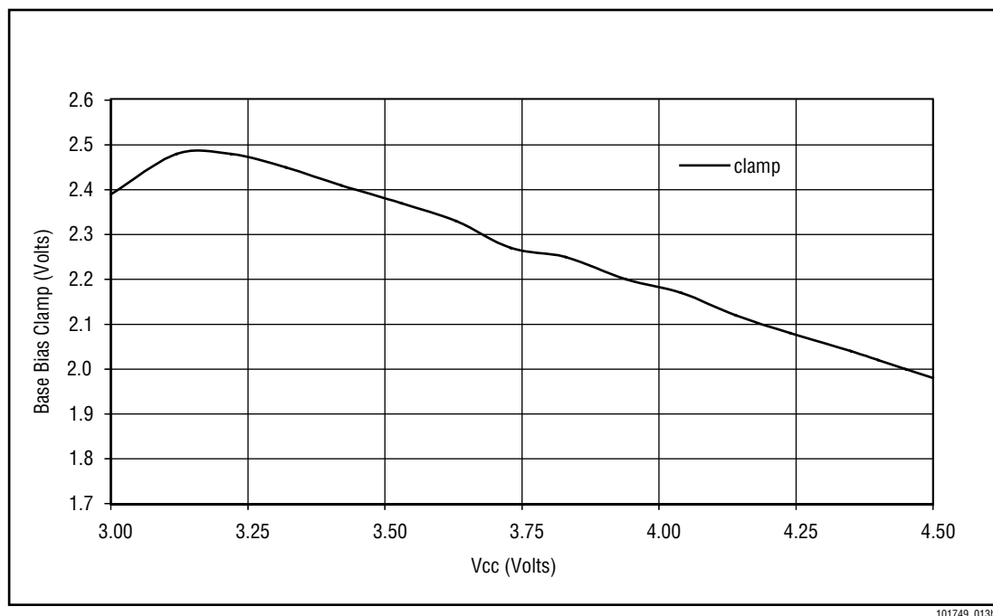
Figure 11. Base Bias Clamp Voltage vs. Supply Voltage
