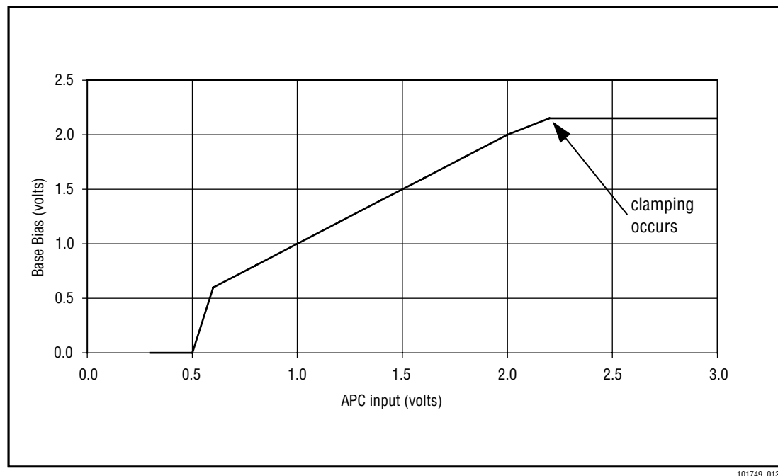
Figure 10. Base Bias Voltage vs. APC Input, V_{CC} = 4.0 V
