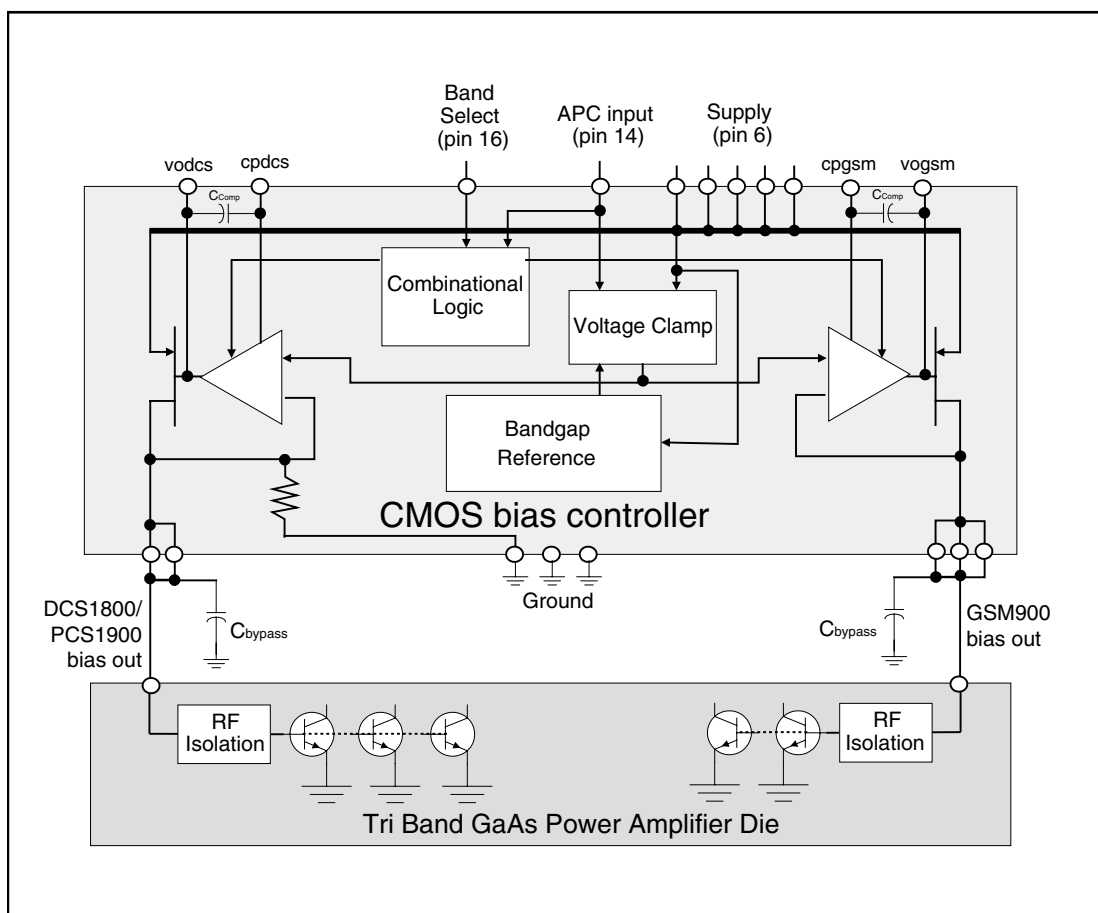
Figure 9. Functional Block Diagram
