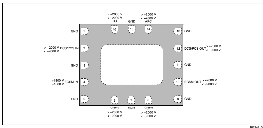
Figure 8. ESD Sensitivity Areas (Top View)
