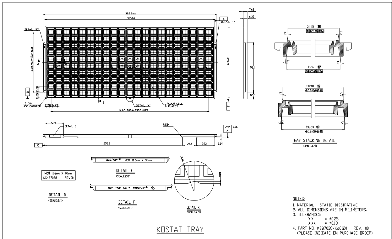
Figure 7. Shipping Tray Dimensions for 9.1mm x 11.6mm Modules
