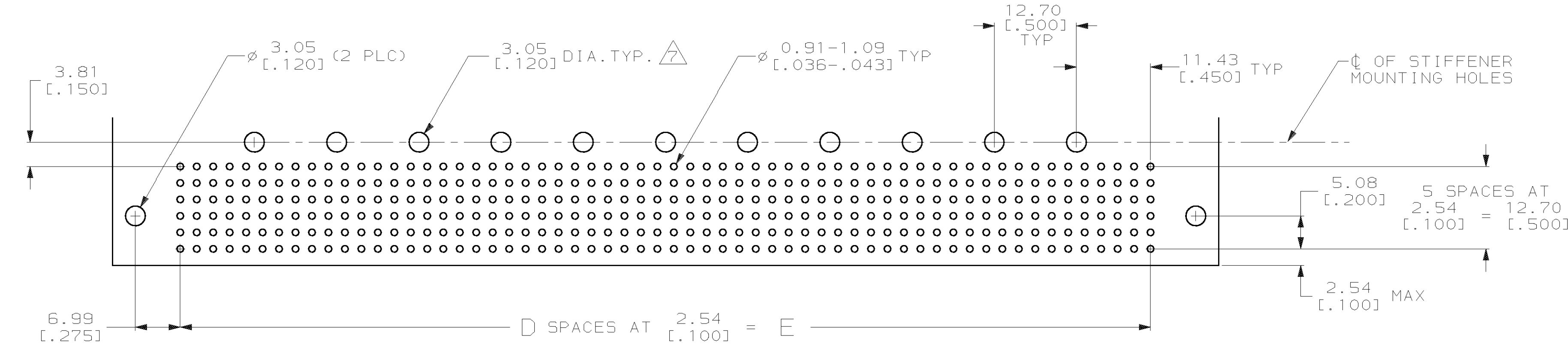
RECOMMENDEC P.C. BOARD LAYOUT
