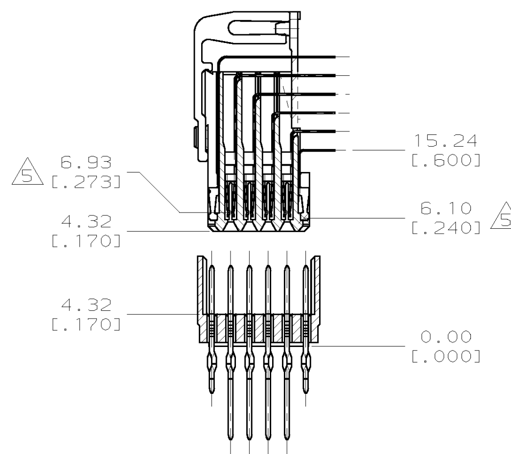
MATING DIMENSIONS REFERENCE
