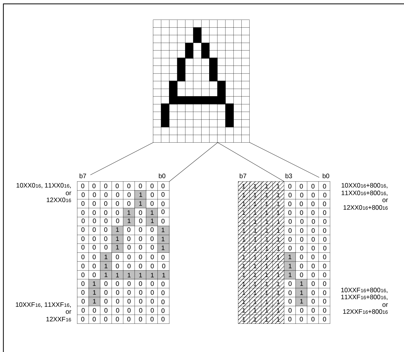
Fig. 52. Display Character Stored Data
