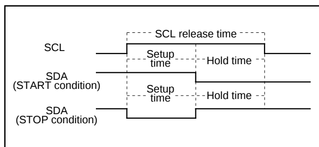
Fig. 33. START Condition/STOP Condition Detect Timing Diagram
