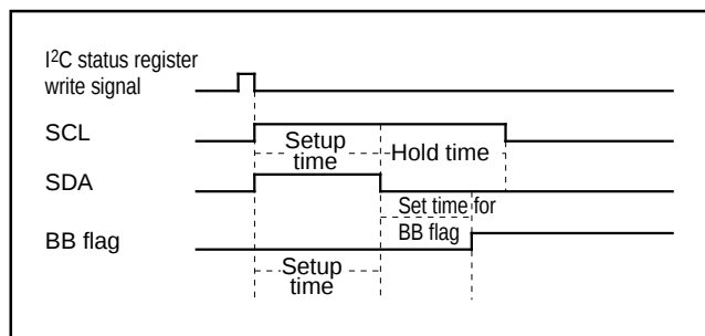
Fig. 31. START Condition Generation Timing Diagram
