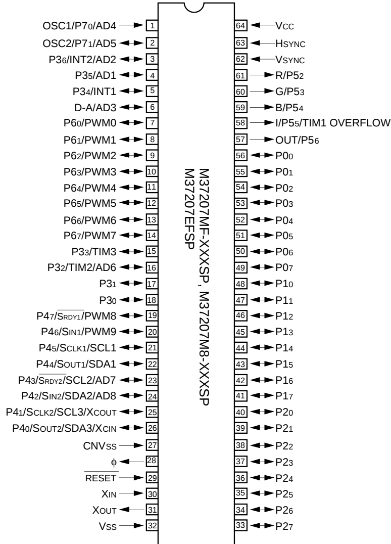
Outline 64P4B
