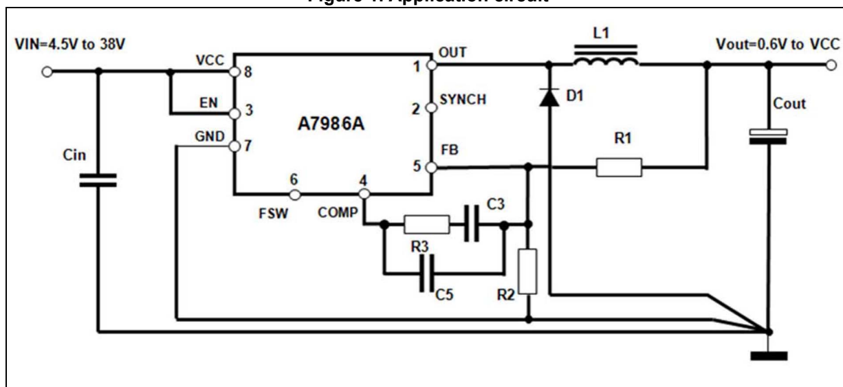
Figure 1. Application circuit
