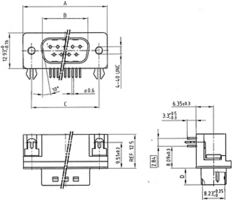
Plug connector
