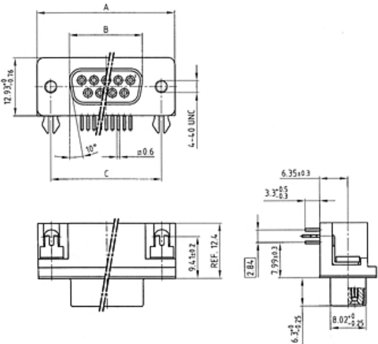
Socket connector
