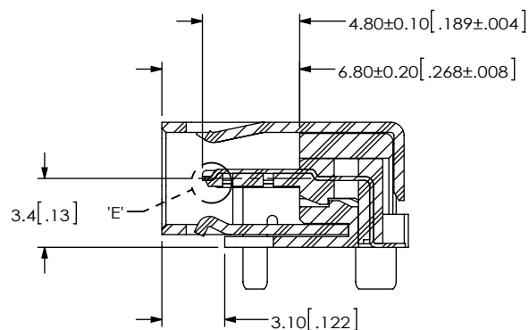
SECTION "D"-"D" SCALE 3 : 1
