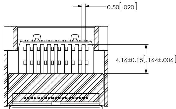
SECTION "B"-"B" SCALE 3 : 1
