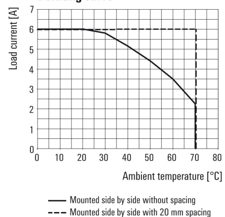
Derating curve
