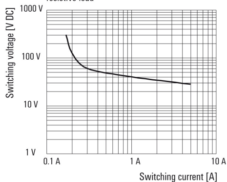
DC load braking capacity resistive load
